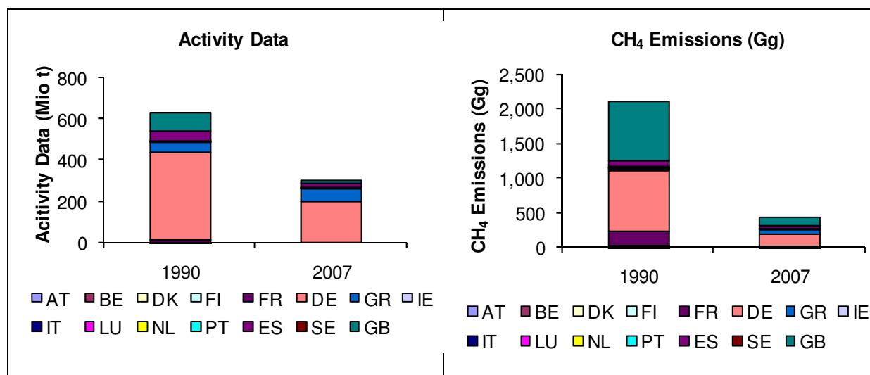
Figure 3.89 1B1a Coal Mining and Handling: Contribution of MS to CH 4 Emission and Activity Data
