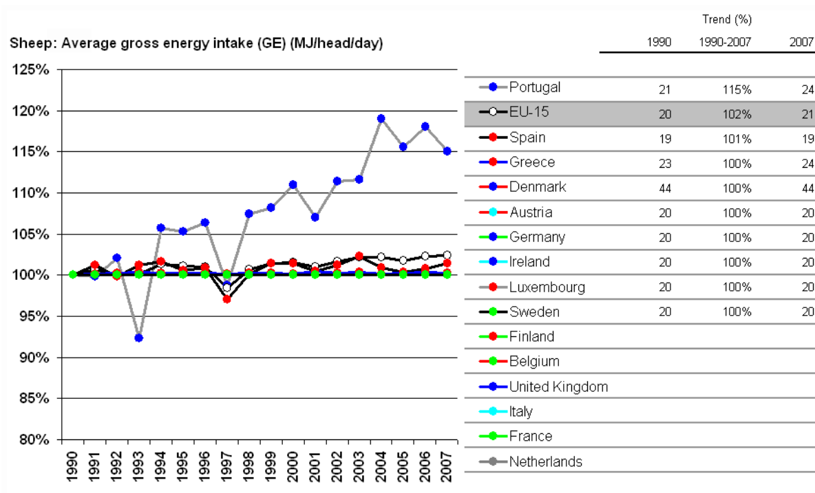
Figure 6.11: Trend of activity data (gross energy intake) for sheep
