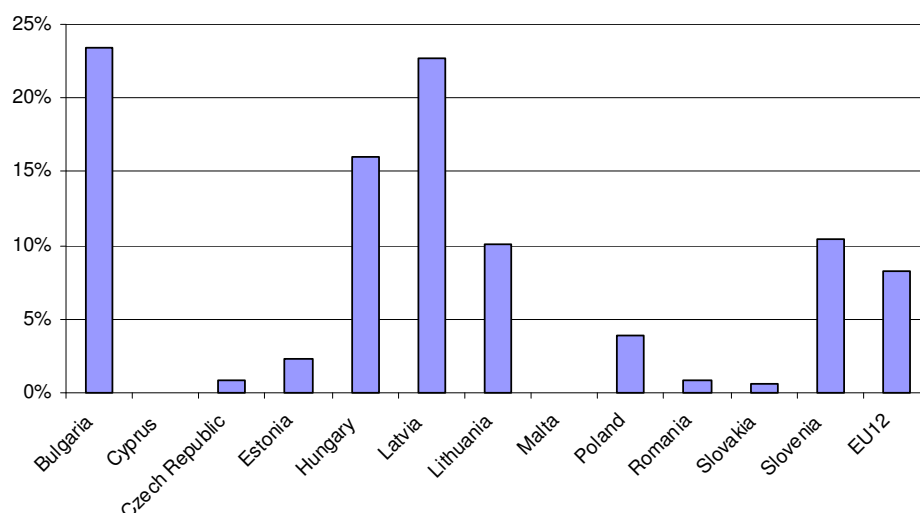
Figure 7.13 The precentual increase of the forest land area between 1990 and 2007(% compared to 1990)
