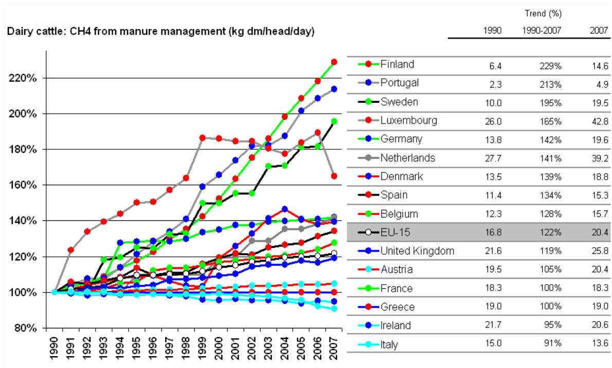
Figure 6.16: Trend of IEF for CH 4 emissions from category 4B(a) for dairy cattle
