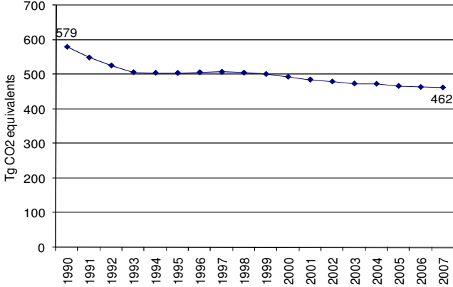
Figure 6.49 Sector 4-Agriculture: EU-27 GHG emissions for 1990–2007 in CO 2 equivalents (Tg)
