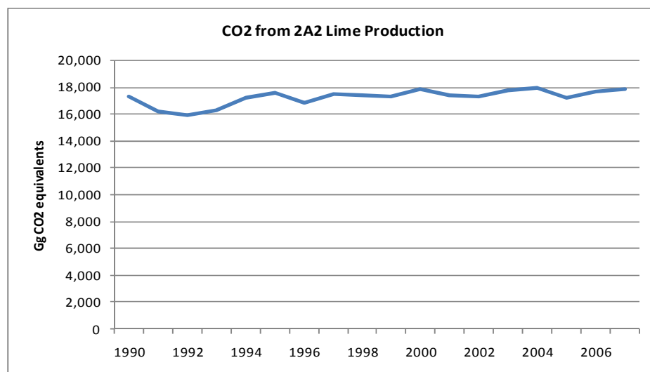
Figure 4.4 2A2 Lime Production: EU-15 CO 2 emissions
