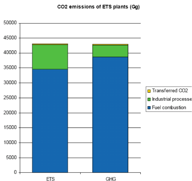
Figure 1.3 CO 2 emissions of ETS plants compared with corresponding emissions reported in the GHG inventories
