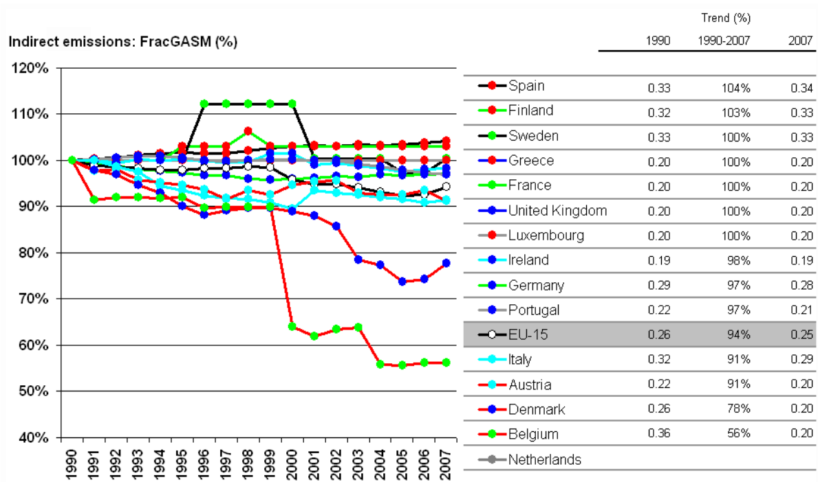
Figure 6.41: Trend of Frac GASM
