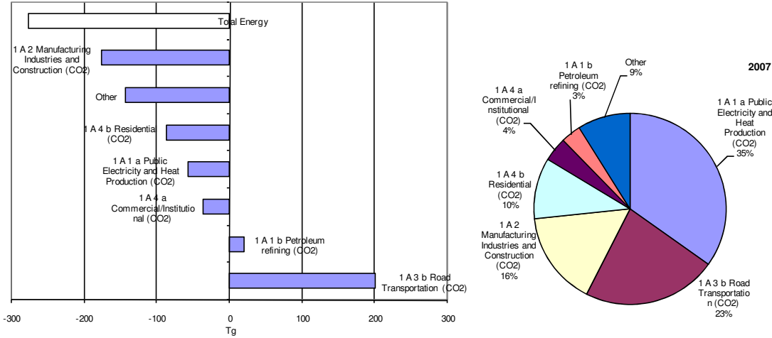
Figure 3.100: CRF Sector 1 Energy: Absolute change of GHG emissions in CO 2 equivalents (Tg) by large key source categories for 1990–2007 and share of largest key source categories in 2007
