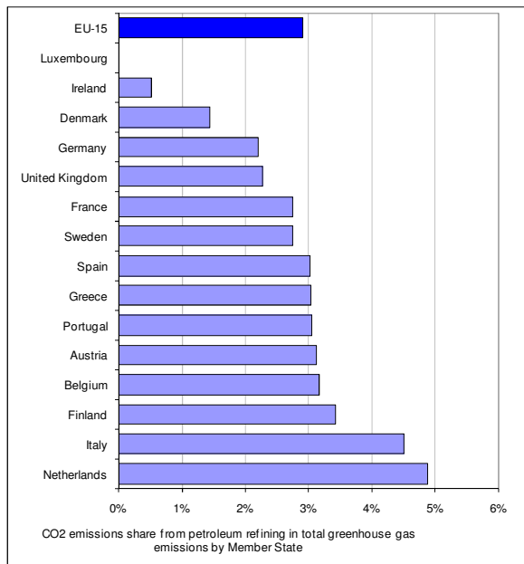
Figure 3.16: Share of CO 2 emissions from petroleum refining in total greenhouse gas emissions by Member State in 2007
