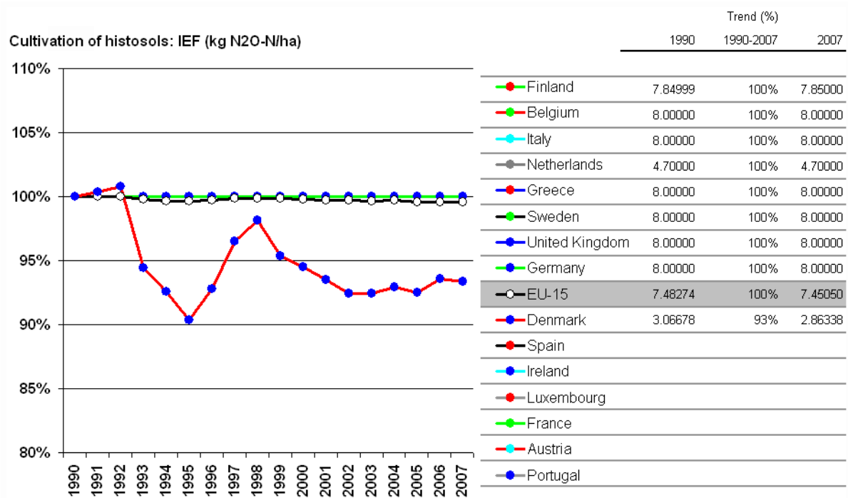
Figure 6.44: Trend of direct emissions from the cultivation of histosols - IEF
