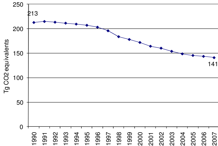
Figure 8.10 Sector 6 Waste: EU-27 GHG emissions 1990–2007 from CRF in CO 2 equivalents (Tg)
