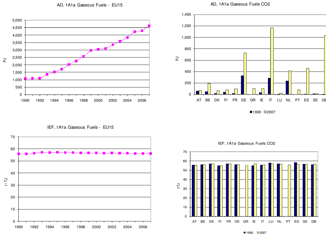
Figure 3.13: 1A1a-Public Electricity and Heat Production, gaseous fuels: Activity Data and Implied Emission Factors for CO 2
