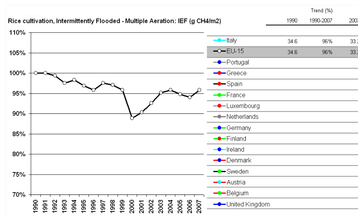
Figure 6.31: Trend of intermittently flooded (multiple aeration) rice cultivation –implied emission factor
