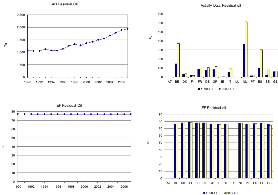
Figure 3.97 Marine bunkers' – Residual Oil:Activity Data and Implied Emission Factors for CO 2
