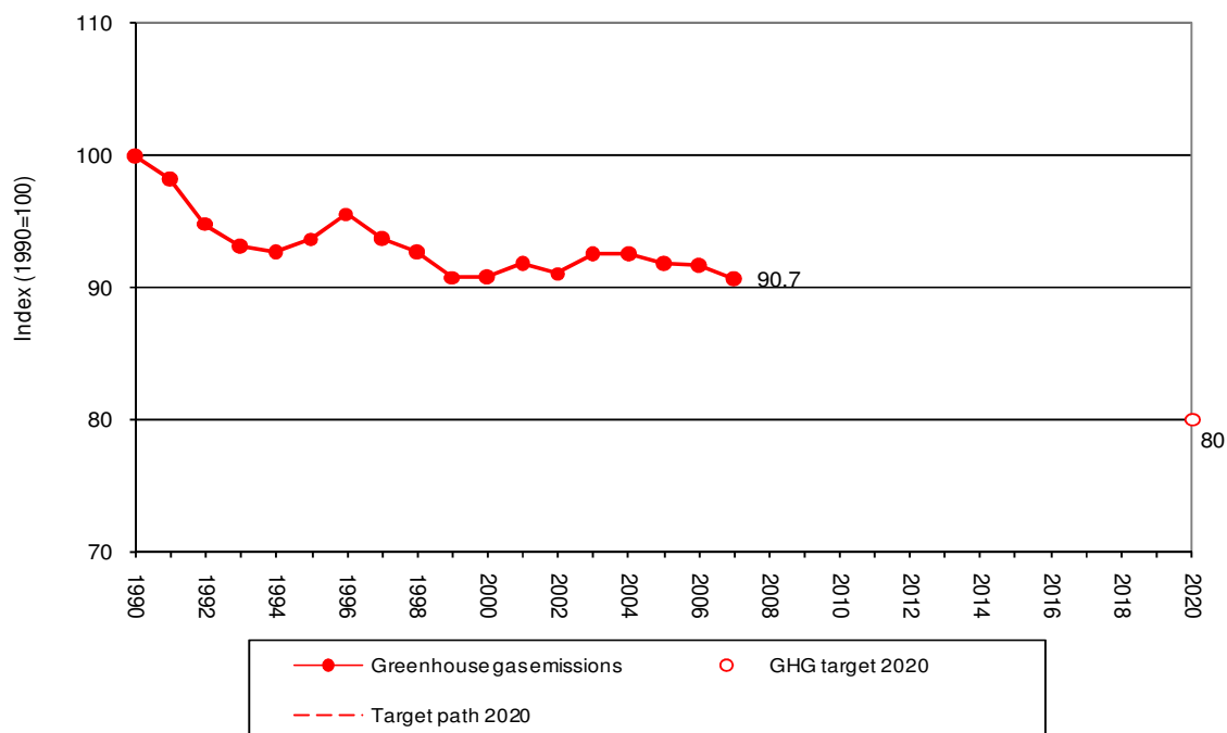
Figure 2.1 EU-27 GHG emissions 1990–2007 (excl. LULUCF)
