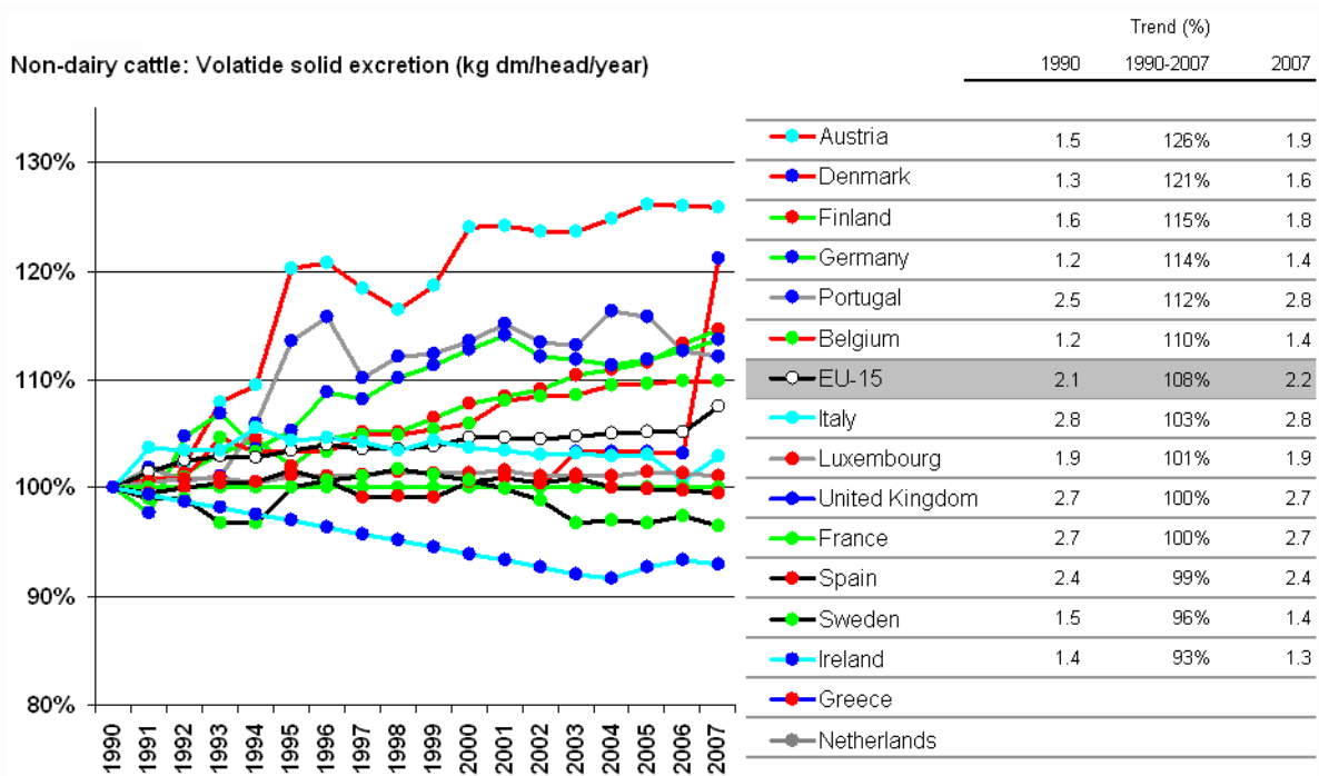
Figure 6.14: Trend of volatile solid excretion for non-dairy cattle
