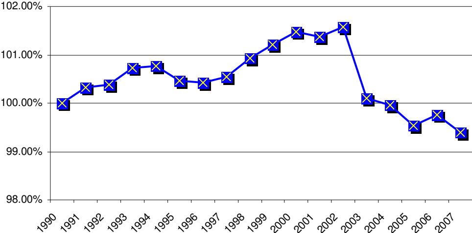
Figure 7.4 The relative trend of Cropland remaining Cropland over the period of 1990-2007 (% relative to 1990)
