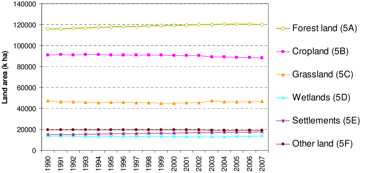
Figure 7.2 EU-15 total land area in the various LULUCF categories (kha), as reported in the Member States' CRFs.
