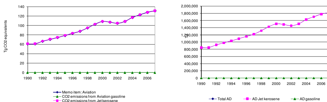
Figure 3.94 Aviation bunkers: Trend of CO 2 Emissions and Activity Data
