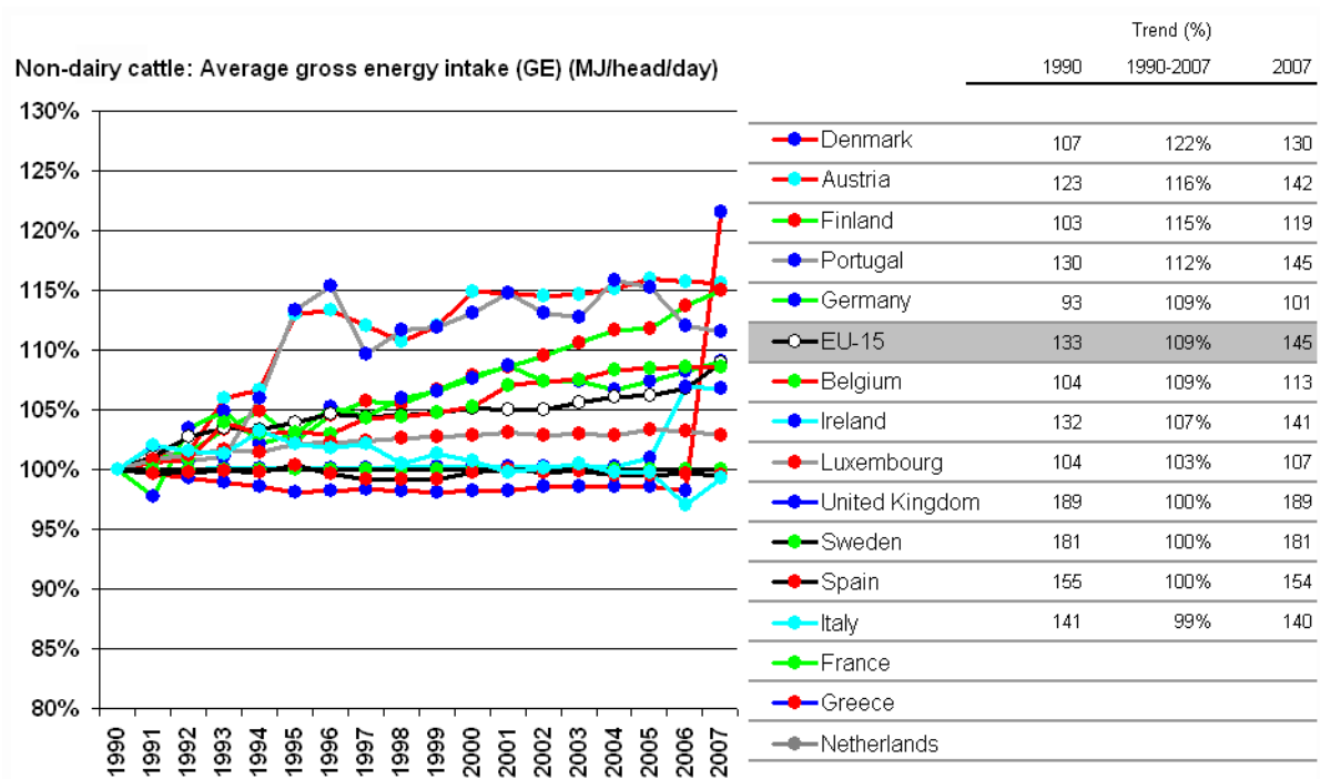
Figure 6.10: Trend of activity data (gross energy intake) for non-dairy cattle.
