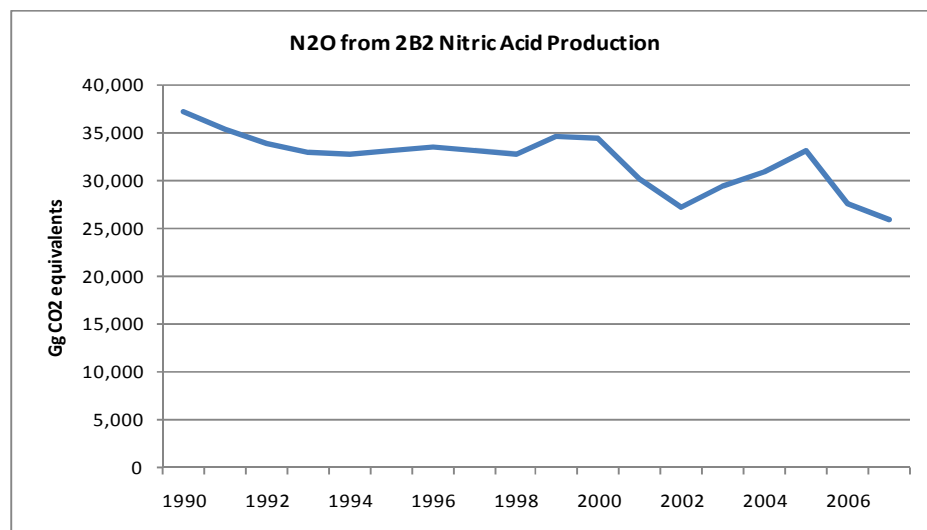
Figure 4.7 2B2 Nitric acid production: EU-15 N 2 O emissions
