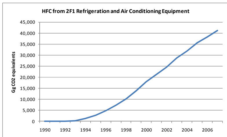
Figure 4.14 2F1 Refrigeration and Air conditioning: EU-15 HFC emissions
