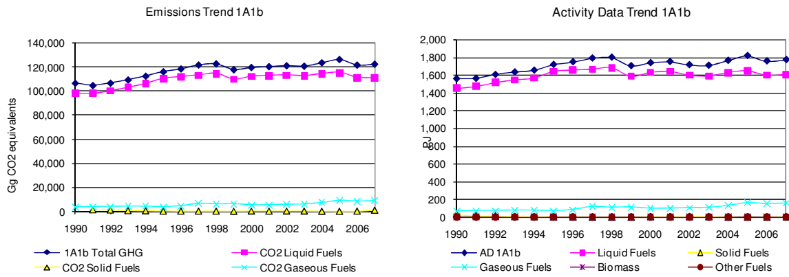
Figure 3.15 1A1b Petroleum Refining: Total and CO 2 emission trends
