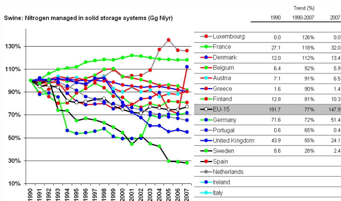
Figure 6.24: Trend of N managed in solid storage and dry lot, swine
