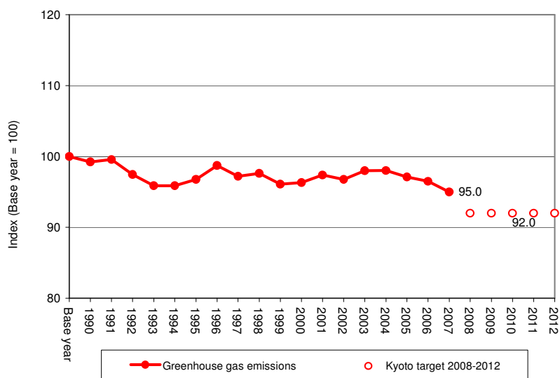
Figure 2.2 EU-15 GHG emissions 1990–2007 compared with target for 2008–12 (excl. LULUCF)
