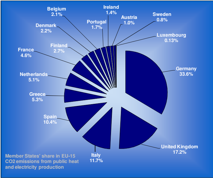
Figure 3.9: Member States' share of CO 2 emissions from public heat and electricity production in EU-15
