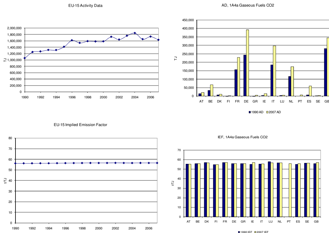
Figure 3.71 1A4a Commercial/Institutional, gaseous fuels: Activity Data and Implied Emission Factors for CO 2
