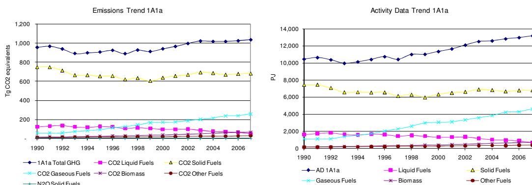
Figure 3.6: 1A1a-Public Electricity and Heat Production: Total, CO 2 and N 2 O emission and activity trends
