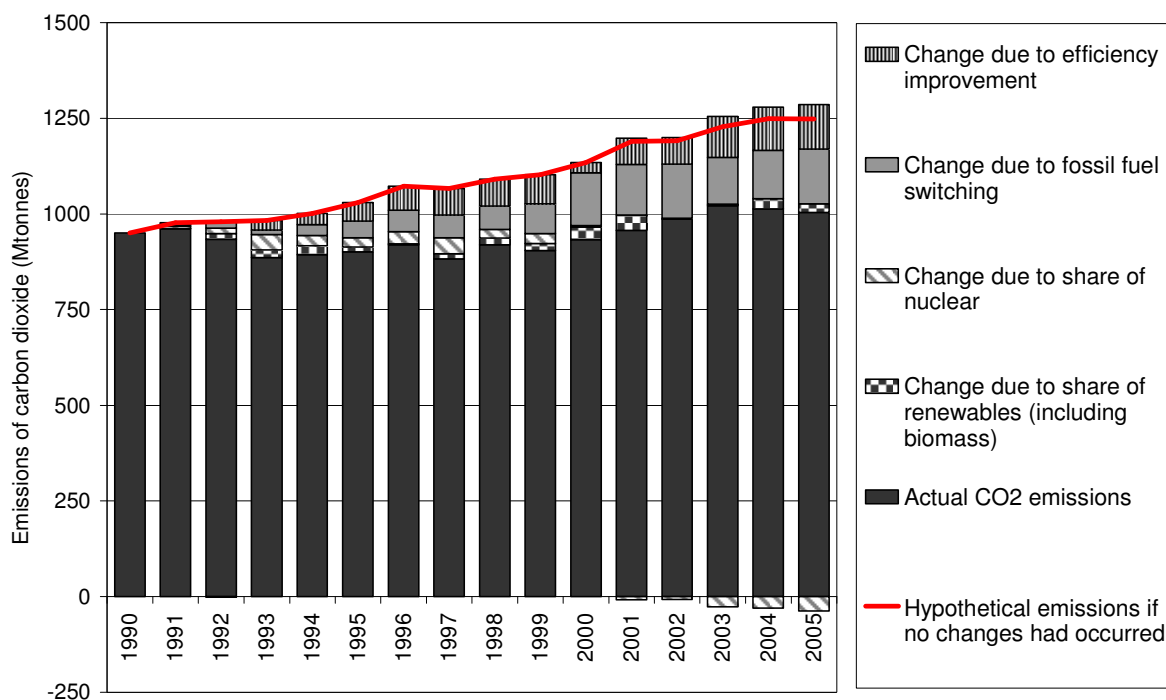
Figure 3.7: Estimated impact of different factors on the reduction in emissions of CO 2 from public electricity and heat production in the EU-15 between 1990 and 2005.
