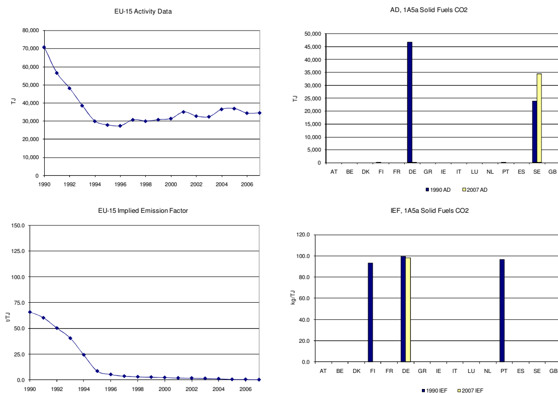
Figure 3.83 1A5a Stationary, solid fuels: Activity Data and Implied Emission Factors for CO 2
