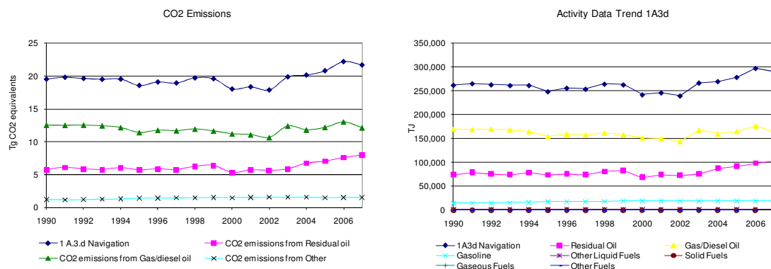
Figure 3.64 1A3d Navigation: CO 2 Emission Trend
