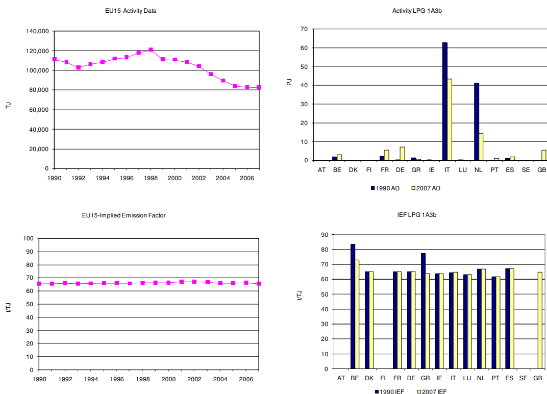
Figure 3.57 1A3b Road Transport, LPG: Activity data and implied emission factors for CO 2
