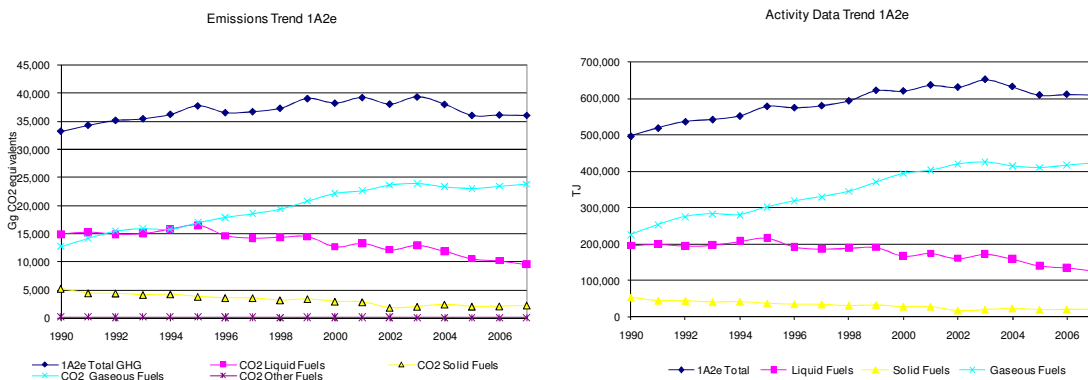
Figure 3.43 1A2e Food Processing, Beverages and Tobacco: Total and CO 2 emission trends
