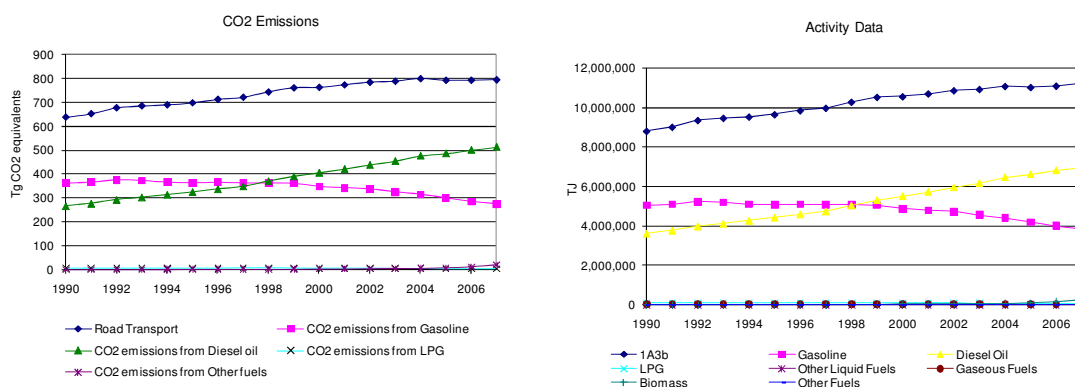
Figure 3.54 1A3b Road Transport: CO 2 Emission Trend and Activity Data
