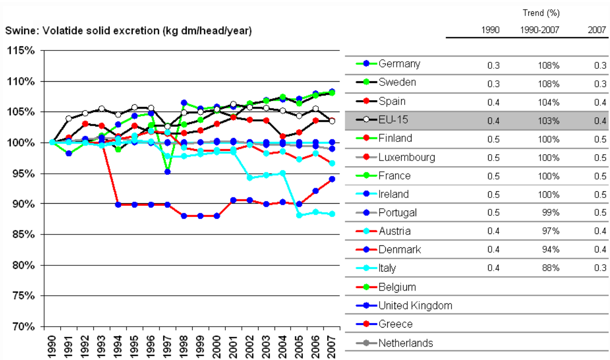
Figure 6.15: Trend of volatile solid excretion for swine
