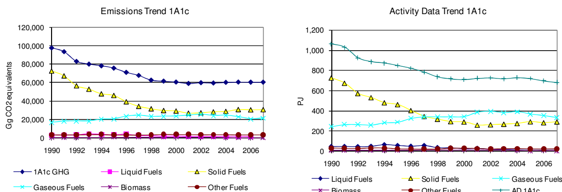
Figure 3.21 1A1c-Manufacture of Solid Fuels and Other Energy Industries: Total and CO 2 emission and activity trends
