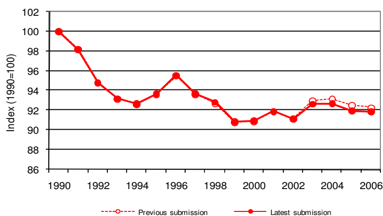
Figure 10.2 Comparison of EU-27 GHG emission trends 1990–2005 (excl. LUCF) of the latest and the previous submission
