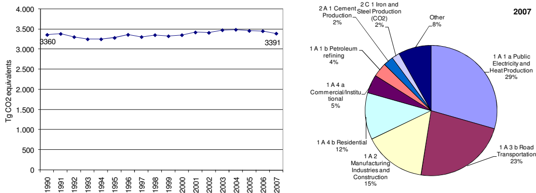
Figure 2.3 CO 2 emissions without LULUCF 1990 to 2007 in CO 2 equivalents (Tg) and share of largest key source categories in 2007 for EU-15
