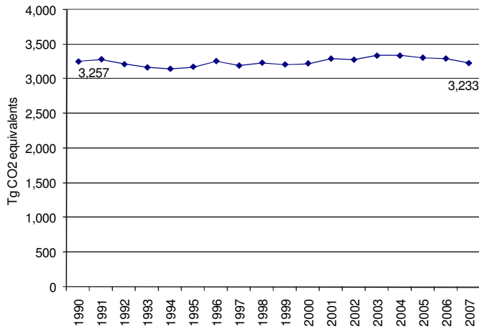
Figure 3.1 CRF Sector 1 Energy: EU-15 GHG emissions in CO 2 equivalents (Tg)for 1990–2007
