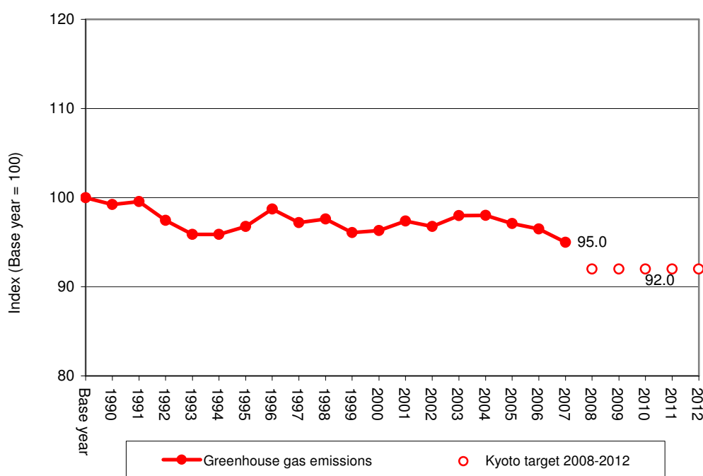
Figure ES.2 EU-15 GHG emissions 1990–2007 (excluding LULUCF) compared with the target for 2008–12
