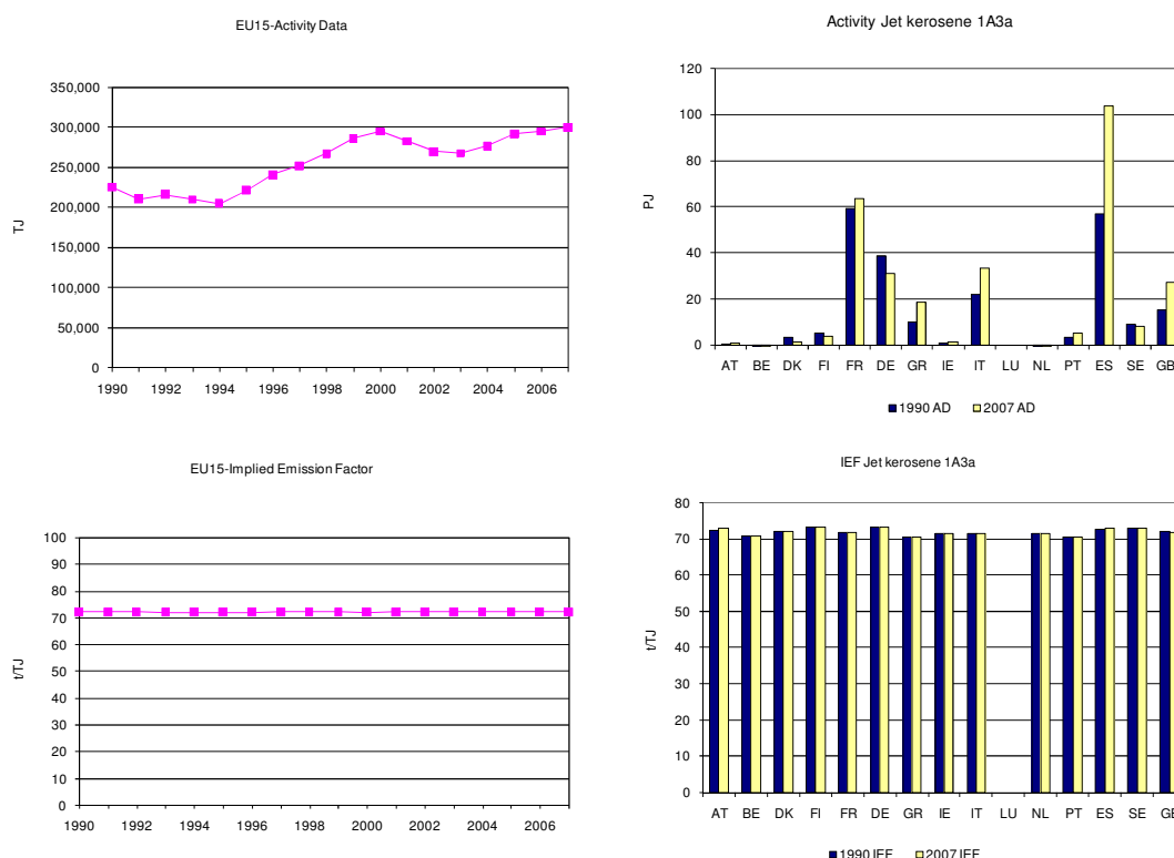
Figure 3.53 1A3a Civil Aviation, jet kerosine: Activity data and implied emission factors for CO 2
