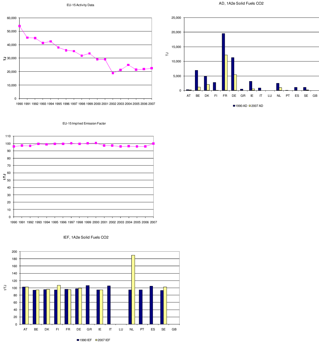
Figure 3.45 1A2e Food Processing, Beverages and Tobacco, solid fuels: Activity Data and Implied Emission Factors for CO 2
