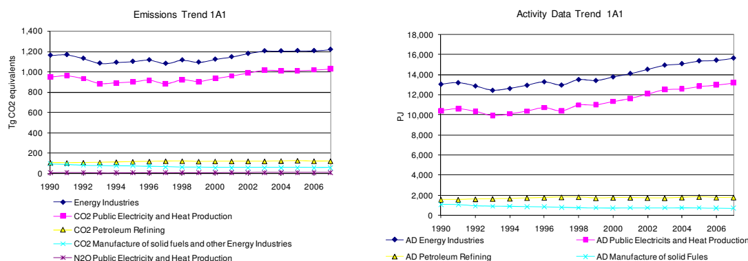
Figure 3.3: 1A1 Energy Industries: Total GHG, CO 2 and N 2 O emission trends and Activity Data
