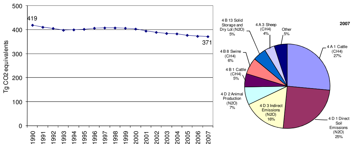
Figure 6.1 EU-15 GHG emissions for 1990–2007 from CRF Sector 4: ‘Agriculture’ in CO 2 equivalents (Tg) and share of largest key source categories in 2007
