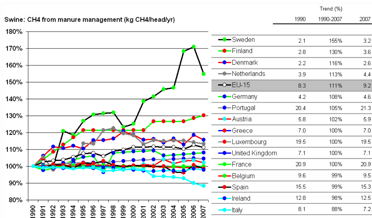
Figure 6.18: Trend of IEF for CH 4 emissions from category 4B(a) for swine
