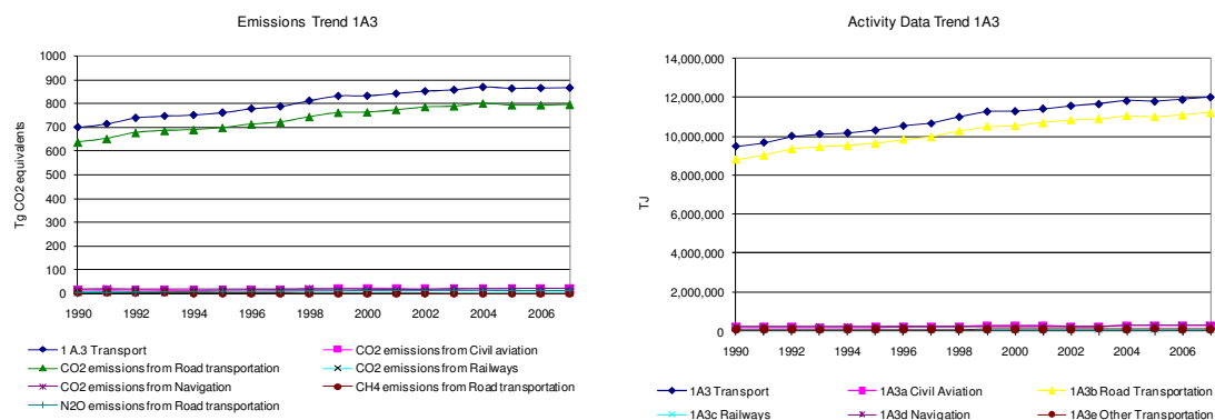
Figure 3.51 1A3 Transport: Greenhouse gas emissions in CO 2 equivalents (Tg) and Activity Data in TJ
