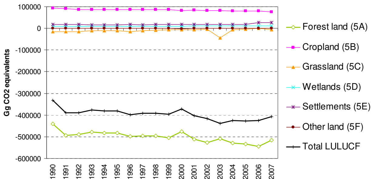
Figure 7.12 Sector 5 LULUCF: EU-27 net CO 2 GHG emissions for 1990–2007 from CRF tables in CO 2 equivalents (Gg)
