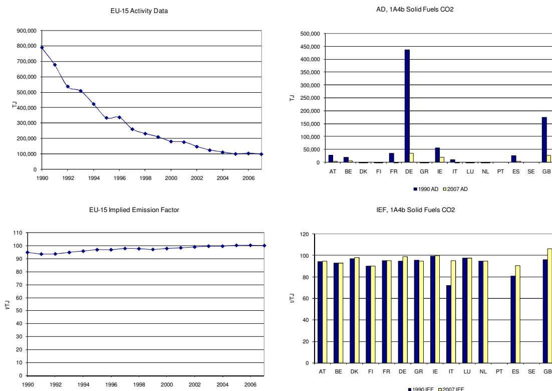
Figure 3.74 1A4b Residential, solid fuels: Activity Data and Implied Emission Factors for CO 2
