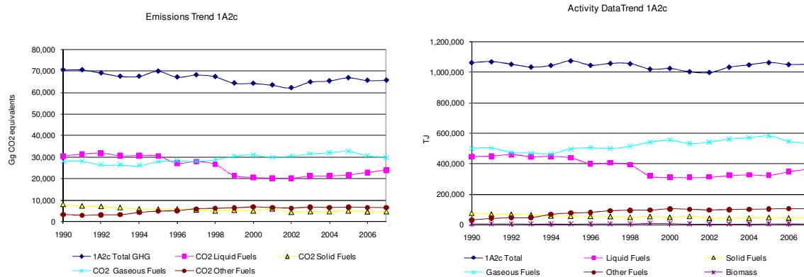
Figure 3.34 1A2c Chemicals: Total and CO 2 emission and activity trends
