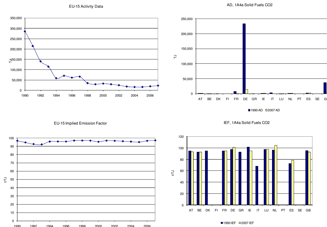
Figure 3.70 1A4a Commercial/Institutional, solid fuels: Activity Data and Implied Emission Factors for CO 2
