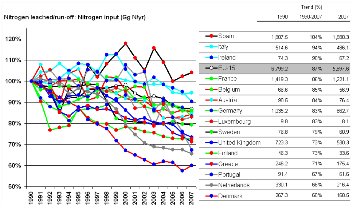
Figure 6.39: Trend of N 2 O emissions for nitrogen leaching and run-off – N-input
