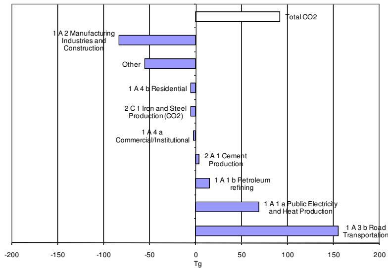
Figure 2.4 Absolute change of CO 2 emissions by large key source categories 1990 to 2007 in CO 2 equivalents (Tg) for EU-15
