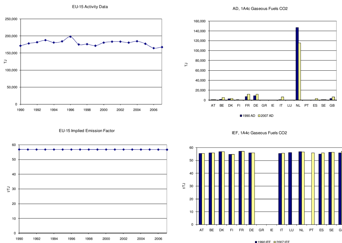
Figure 3.80 1A4c Agriculture/Forestry/Fisheries, gaseous fuels: Activity Data and Implied Emission Factors for CO 2
