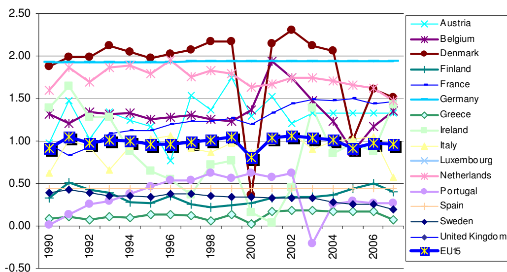
Figure 7.7 Implied net carbon stock change in living biomass in 5A1 (Mg C/ha/year)
