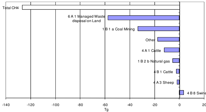
Figure 2.6 Absolute change of CH 4 emissions by large key source categories 1990 to 2007 in CO 2 equivalents (Tg) for EU-15
