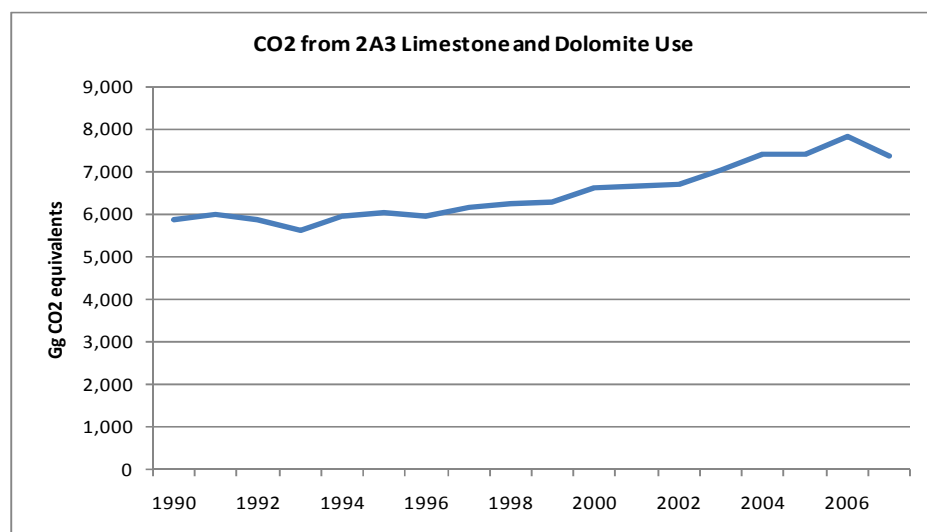
Figure 4.5 2A3 Limestone and Dolomite Use: EU-15 CO 2 emissions
