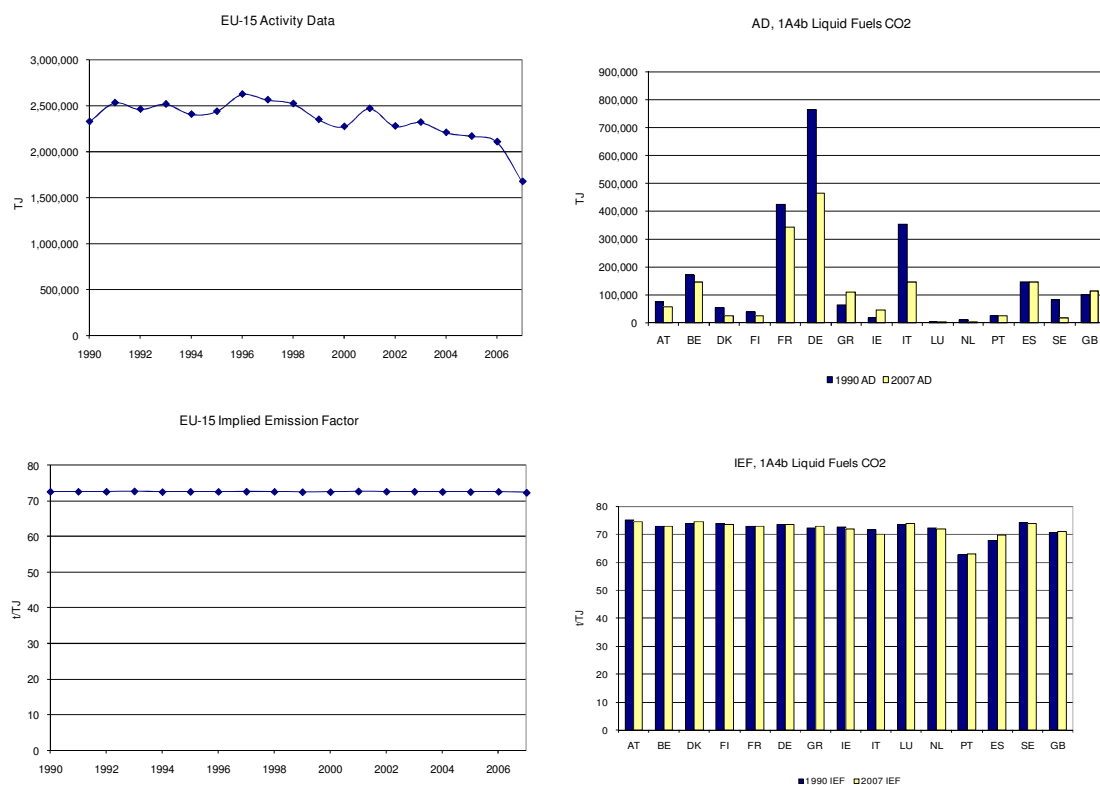
Figure 3.73 1A4b Residential, liquid fuels: Activity Data and Implied Emission Factors for CO 2
