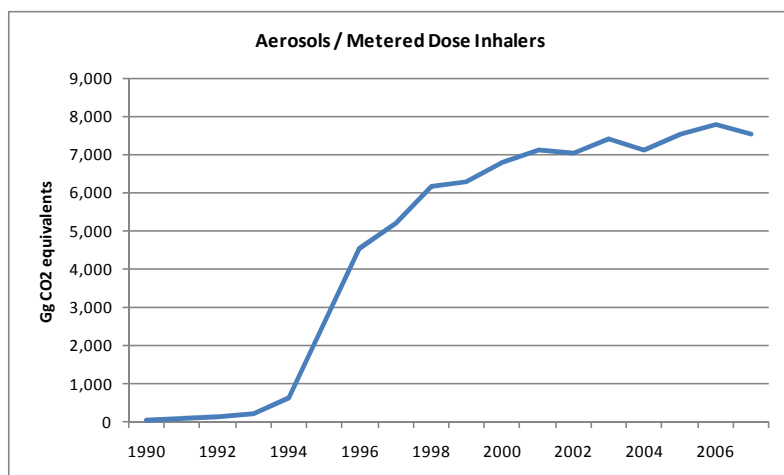
Figure 4.15 2F4 Aerosols/Metered Dose Inhalers: EU-15 HFC emissions
