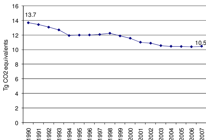
Figure 5.1 Sector 3 Solvent and Other Product Use: EU-15 GHG emissions for 1990–2007 in CO 2 equivalents (Tg)
