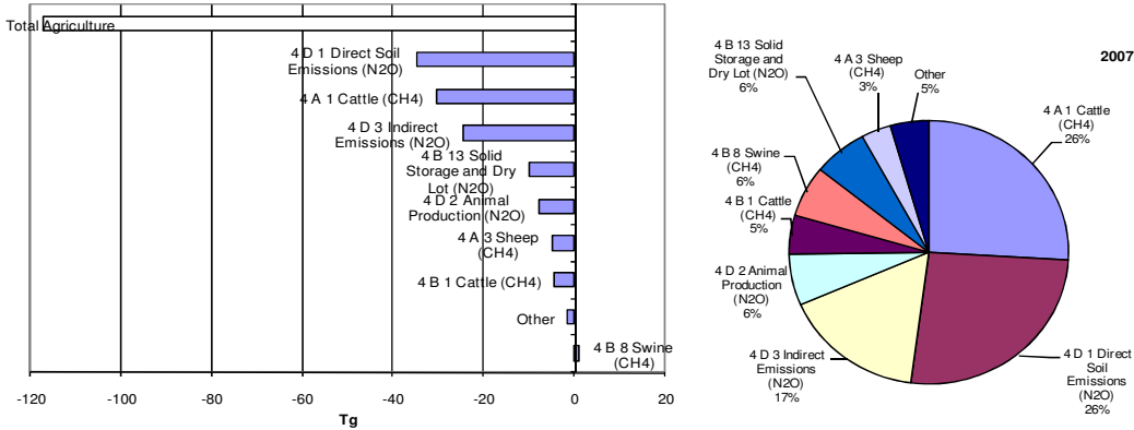
Figure 6.50 Sector 4-Agriculture: Absolute change of GHG emissions by large key source categories 1990–2007 in CO 2 equivalents (Tg) and share of largest key source categories in 2007
