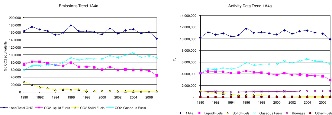
Figure 3.68 1A4a Commercial/Institutional: Total and CO 2 emission and activity trends
