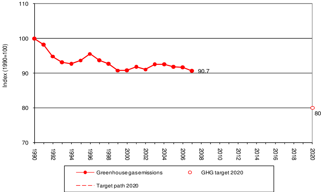
Figure ES.1 EU-27 GHG emissions 1990–2007 (excluding LULUCF)
