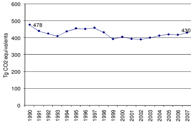
Figure 4.17 CRF Sector 2 Industrial Processes: EU-27 GHG emissions for 1990–2007 in CO 2 equivalents (Tg)
