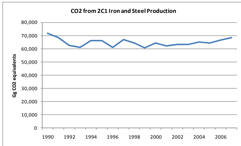
Figure 4.11 2C1 Iron and Steel Production: EU-15 CO 2 emissions
