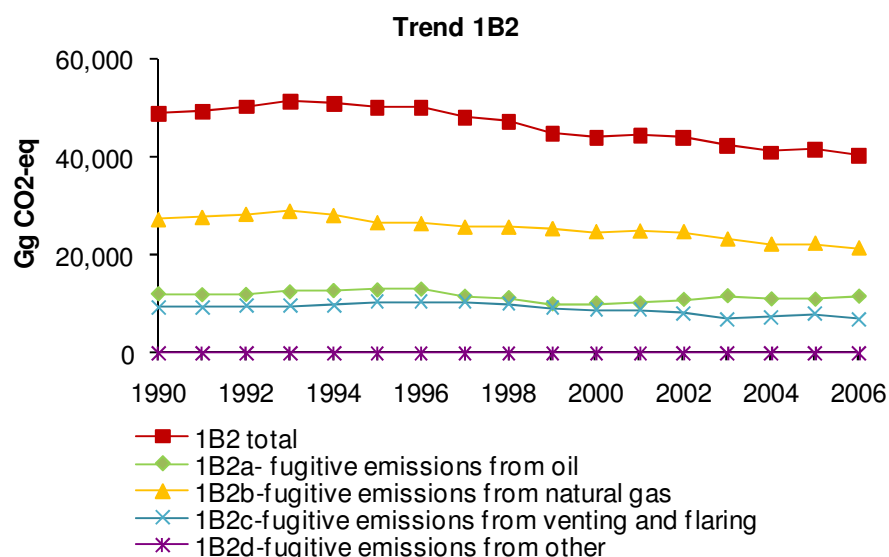
Figure 3.92 1B2-Fugitive Emissions Oil and Natural Gas: Trend
