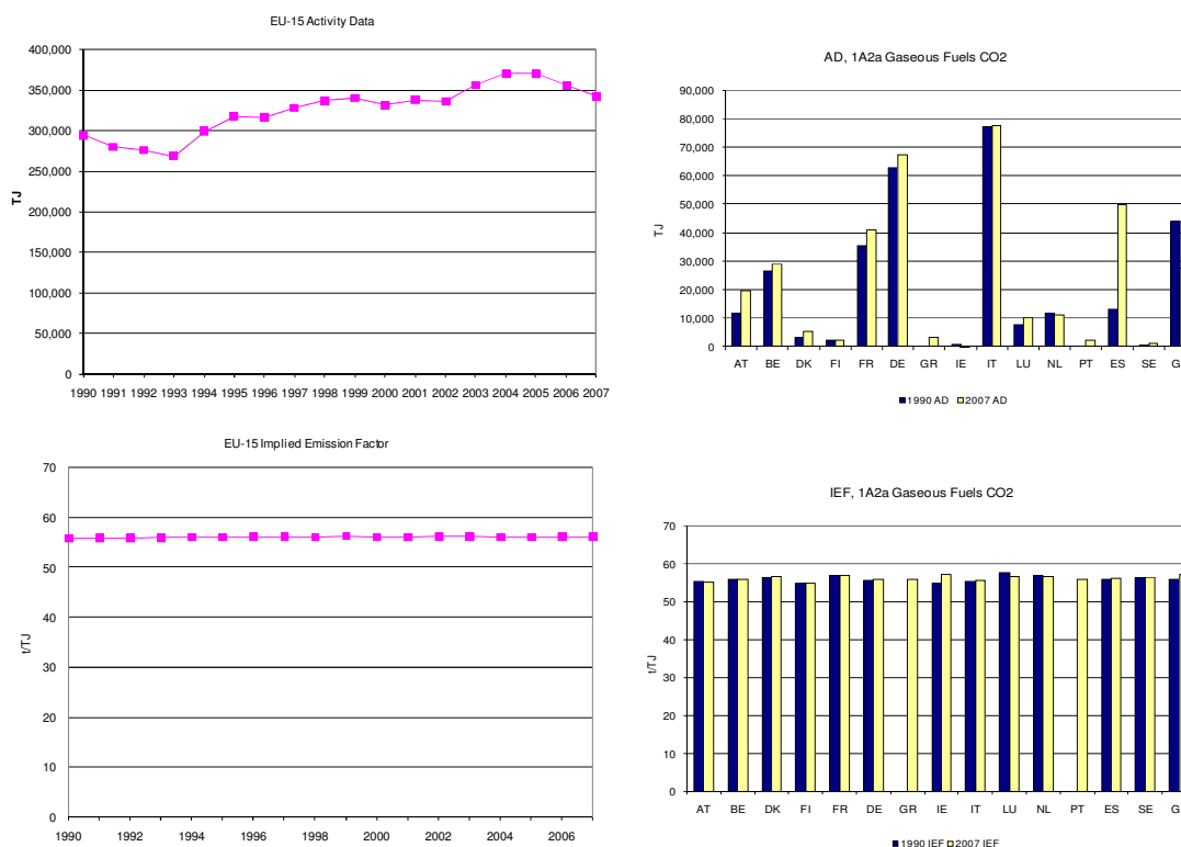
Figure 3.30 1A2a Iron and Steel, gaseous fuels: Activity Data and Implied Emission Factors for CO 2
