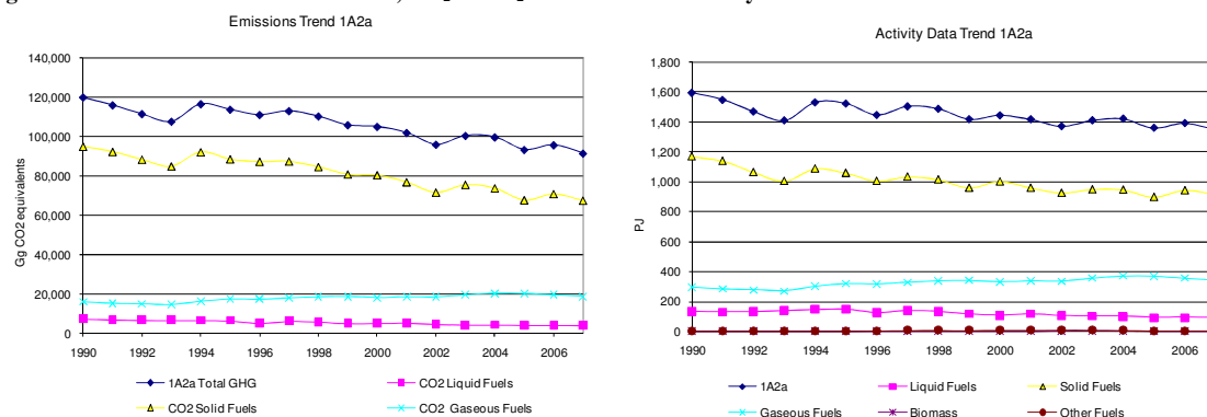
Figure 3.27 1A2a Iron and Steel: Total, CO 2 and N 2 O emission and activity trends
