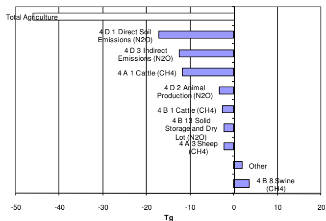
Figure 6.2 Absolute change of GHG emissions by large key source categories 1990–2007 in CO 2 equivalents (Tg) in CRF Sector 4: ‘Agriculture’
