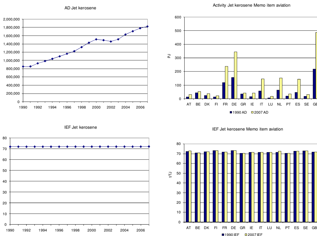
Figure 3.95 Aviation bunkers, Jet kerosene: Activity Data and Implied Emission Factors for CO 2
