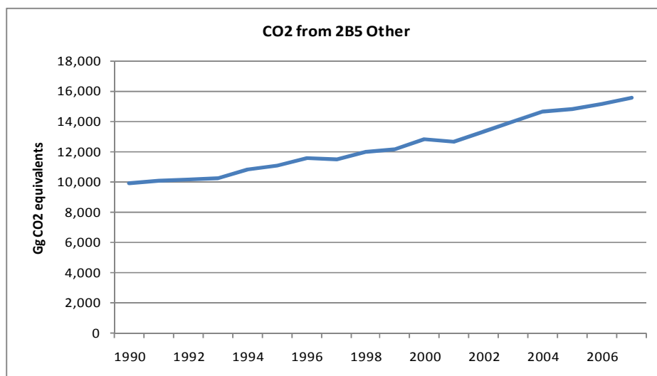
Figure 4.9 2B5 Other: EU-15 CO 2 emissions
