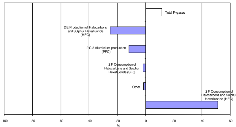
Figure 2.10 Absolute change of fluorinated gas emissions by large key source categories 1990 to 2007 in CO 2 equivalents (Tg) for EU-15
