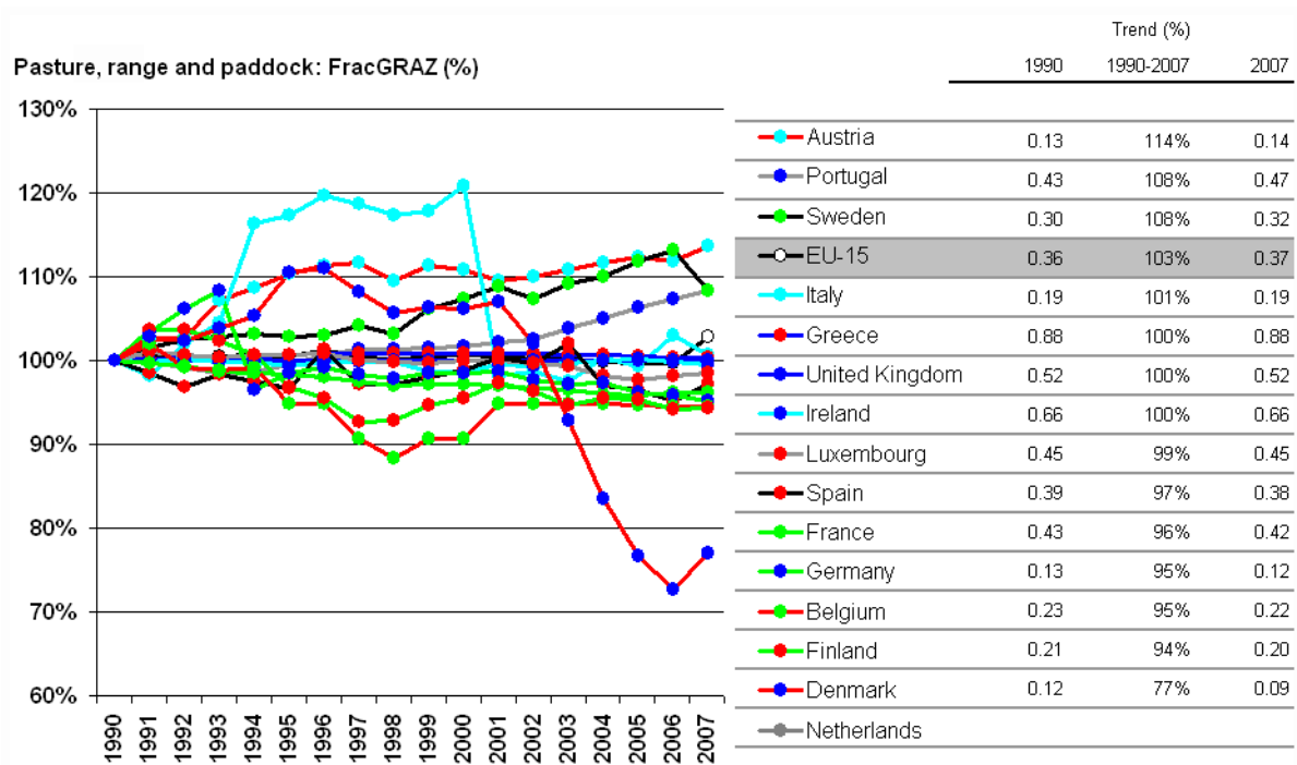
Figure 6.42: Trend of Frac GRAZ
