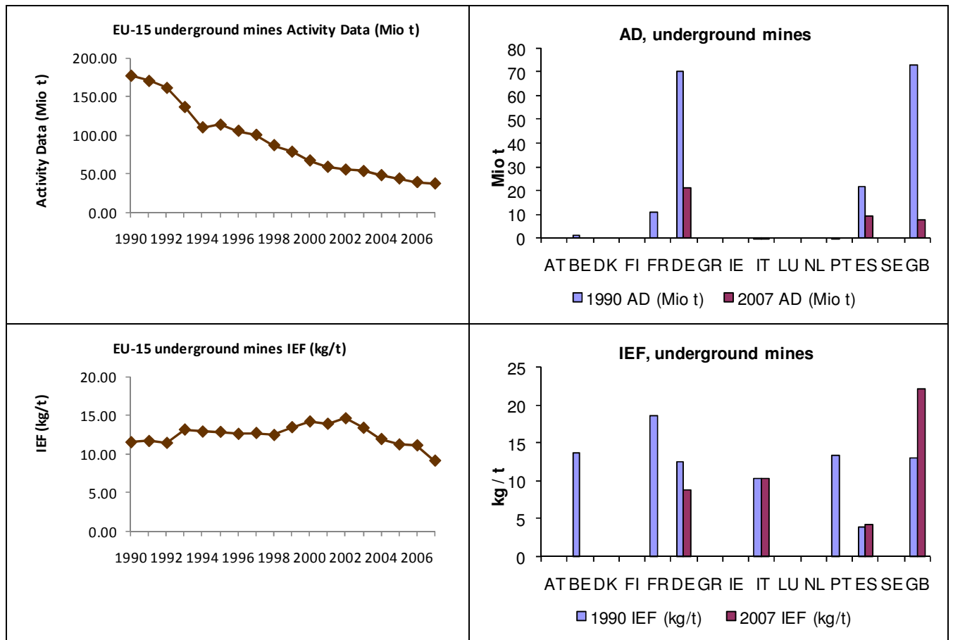
Figure 3.90 1B1ai Underground Mines: Activity Data and Implied Emission Factors for EU-15 and the emitting countries of CH 4
