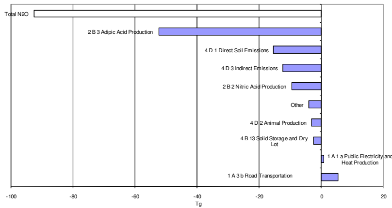
Figure 2.8 Absolute change of N 2 O emissions by large key source categories 1990 to 2007 in CO 2 equivalents (Tg) for EU-15
