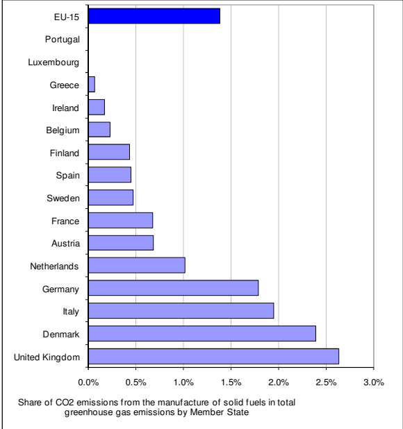
Figure 3.23: Member States' share of CO 2 emissions from the manufacture of solid fuels in EU-15
