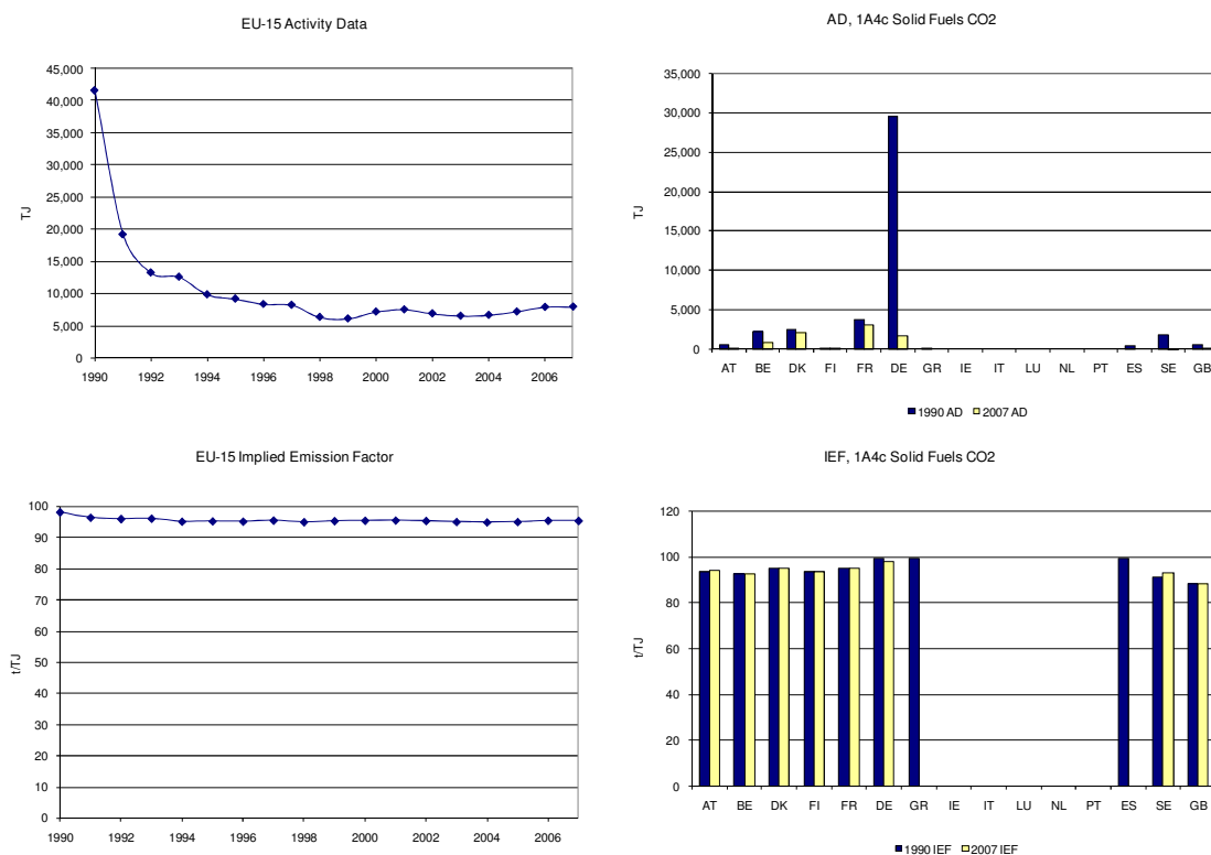
Figure 3.79 1A4c Agriculture/Forestry/Fisheries, solid fuels: Activity Data and Implied Emission Factors for CO 2
