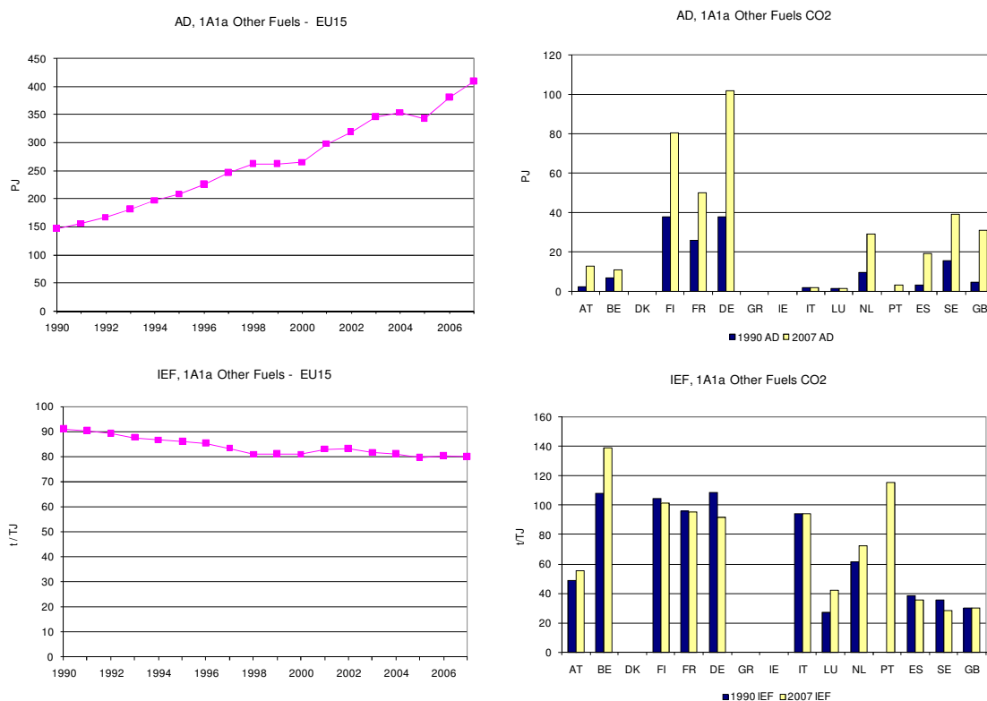
Figure 3.14: 1A1a Public Electricity and Heat Production, other fuels: Activity Data and Implied Emission Factors for CO 2
