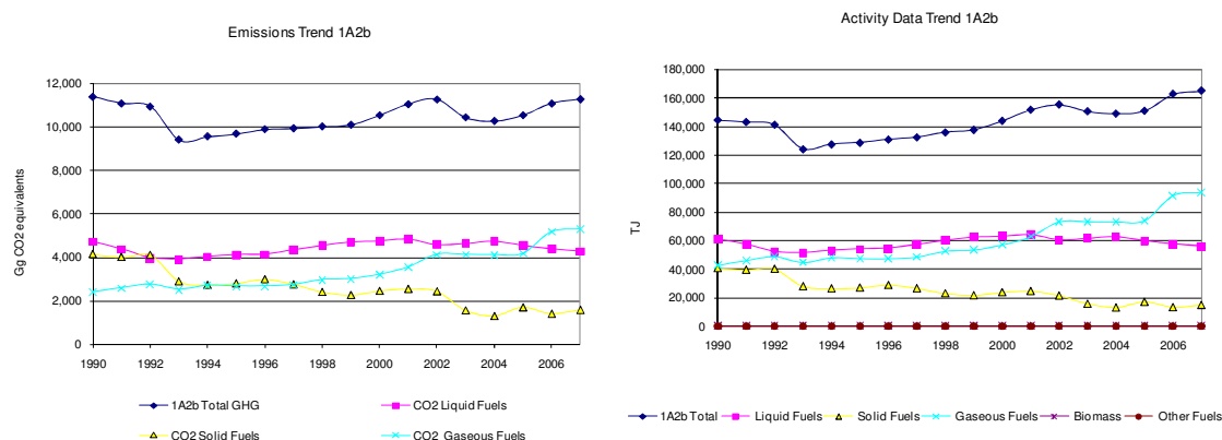
Figure 3.31 1A2b Non ferrous Metals: Total and CO 2 emission trends
