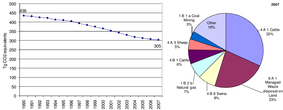
Figure 2.5 CH 4 emissions 1990 to 2007 in CO 2 equivalents (Tg) and share of largest source categories in 2007 for EU-15
