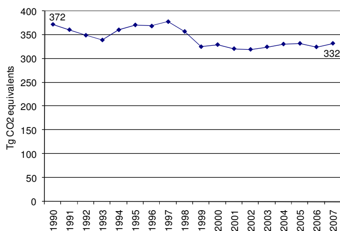
Figure 4.1 CRF Sector 2 Industrial Processes: EU-15 GHG emissions for 1990–2007 in CO 2 equivalents (Tg)
