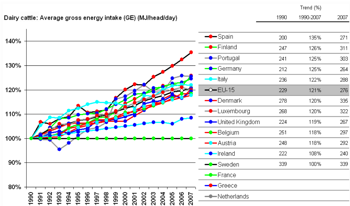
Figure 6.9.: Trend of activity data (gross energy intake) for dairy cattle.
