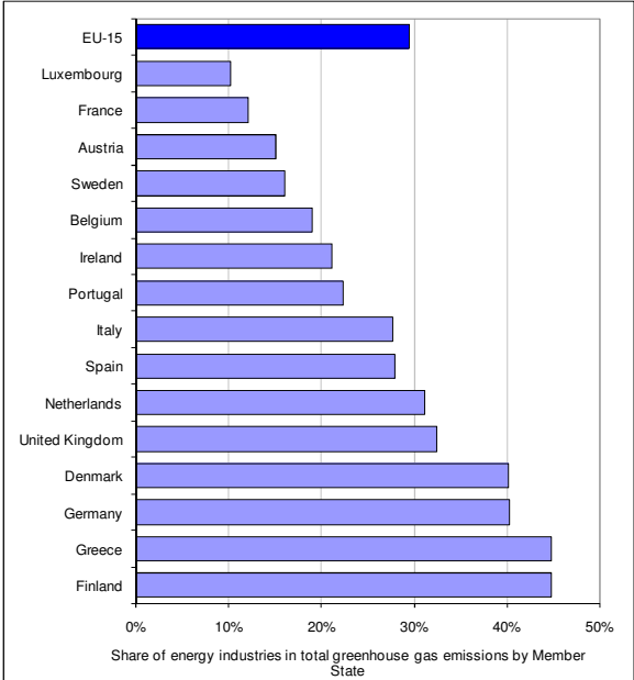
Figure 3.4: Share of greenhouse gas emissions from energy industries in total greenhouse gas emissions by Member State in 2007
