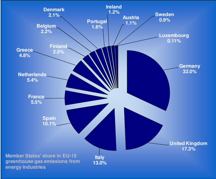
Figure 3.5: Member States’ share of greenhouse gas emissions from energy industries in EU-15
