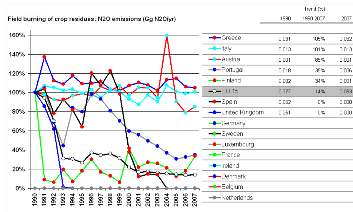
Figure 6.47: Trend of N 2 O emissions from field burning of crop residues
