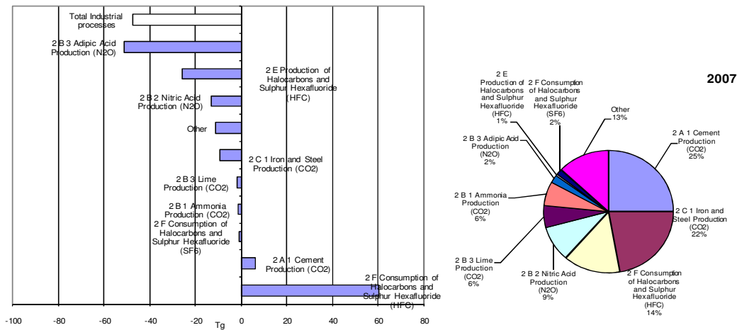
Figure 4.18 CRF Sector 2 Industrial processes: Absolute change of GHG emissions by large key source categories 1990–2007 in CO 2 equivalents (Tg) and share of largest key source categories in 2007
