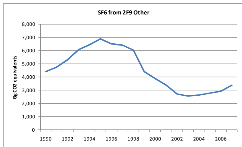
Figure 4.16 2F9 Other: EU-15 SF 6 emissions
