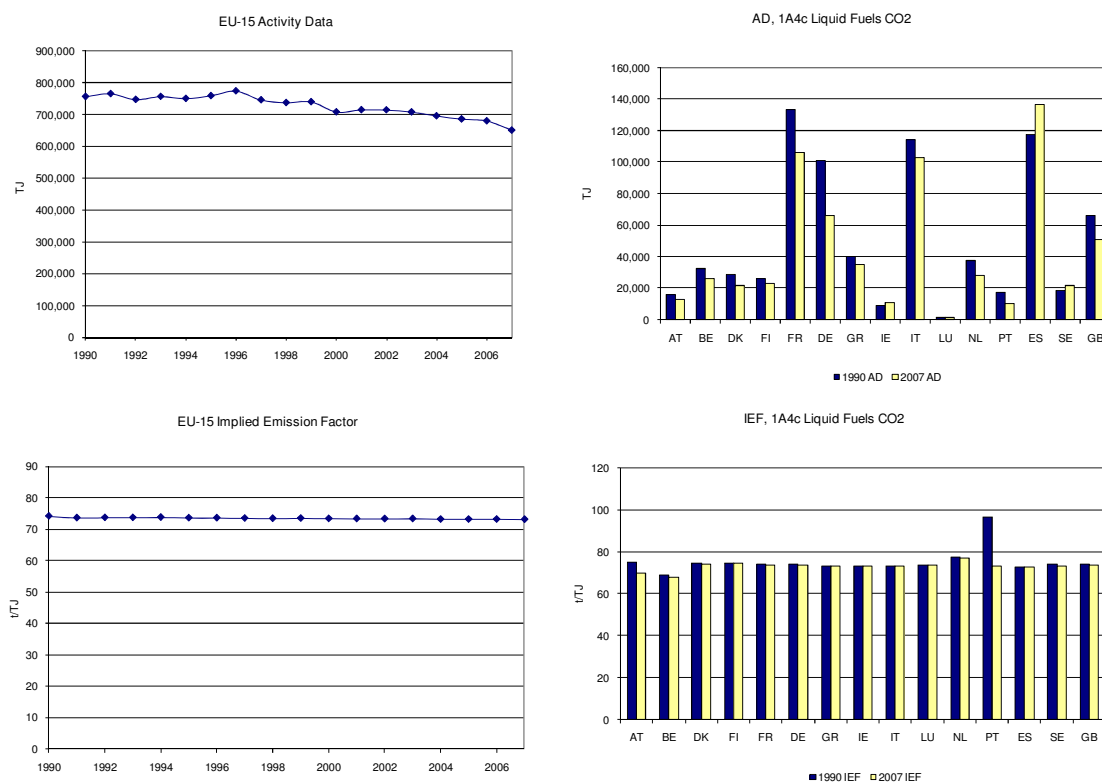
Figure 3.78 1A4c Agriculture/Forestry/Fisheries, liquid fuels: Activity Data and Implied Emission Factors for CO 2
