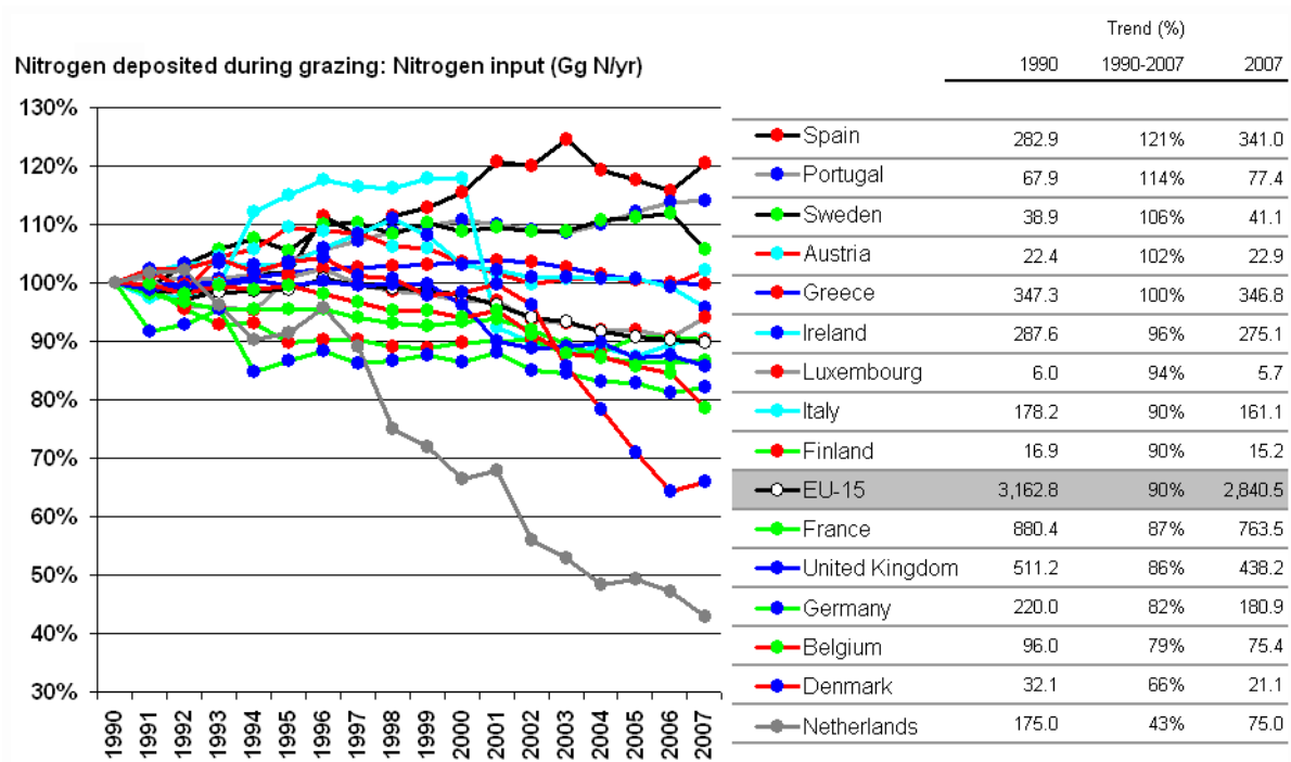
Figure 6.37: Trend of N 2 O emissions from pasture, range, and paddock – N-input
