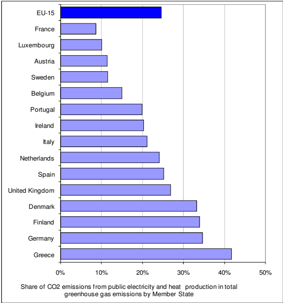
Figure 3.8: Share of CO 2 emissions from public electricity and heat production in total greenhouse gas emissions by Member State in 2007
