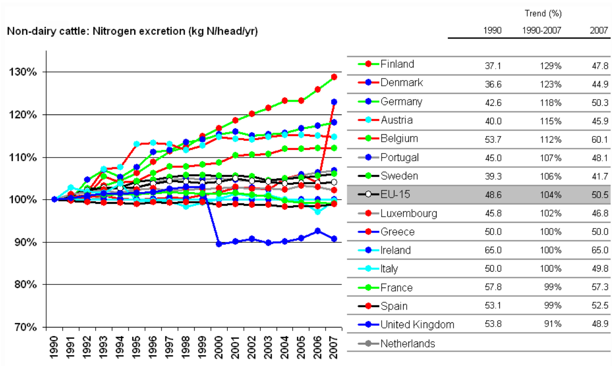
Figure 6.20: Trend of nitrogen excretion rates for non-dairy cattle:
