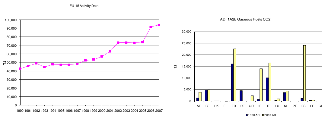
Figure 3.33 1A2b Non ferrous Metals, gaseous fuels: Activity Data and Implied Emission Factors for CO 2
