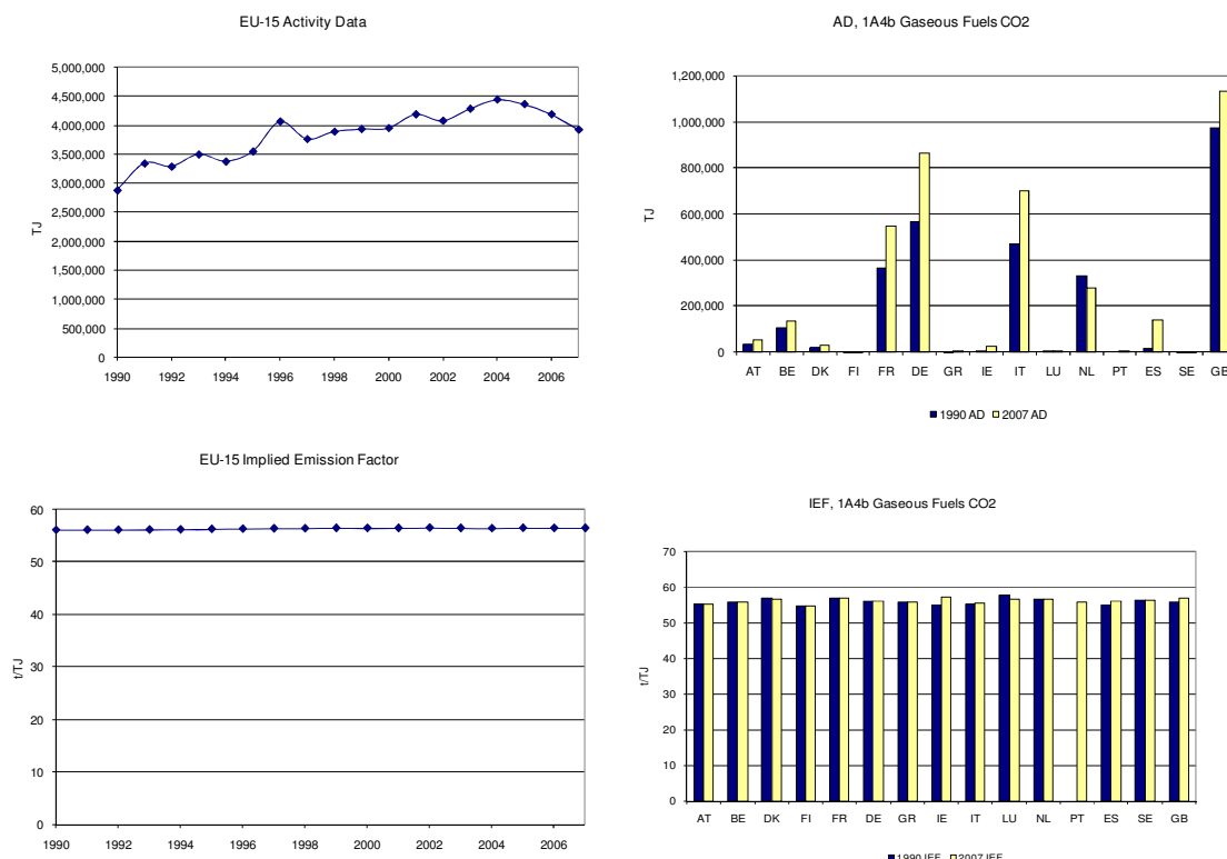
Figure 3.75 1A4b Residential, gaseous fuels: Activity Data and Implied Emission Factors for CO 2
