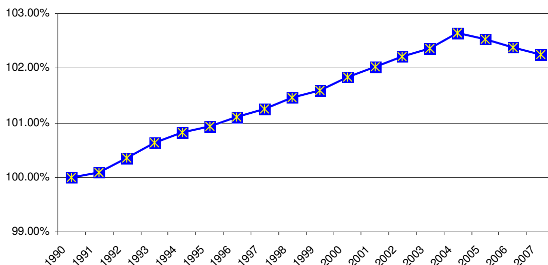
Figure 7.3. Relative trend of area of 5A1 - forest remaining forest in EU-15, 1990-2007
