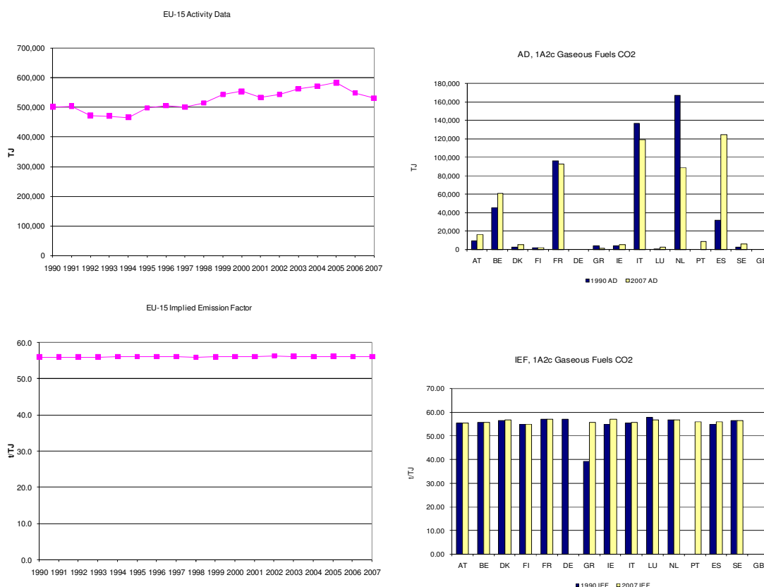
Figure 3.37 1A2c Chemicals, gaseous fuels: Activity Data and Implied Emission Factors for CO 2
