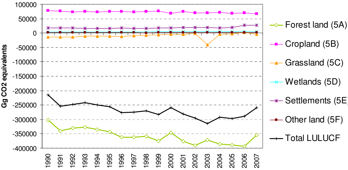
Figure 7.1 Sector 5 LULUCF: EU-15 GHG emissions (+) and removals (-) for 1990–2007, in CO 2 eq. (Gg), for all land use categories.
