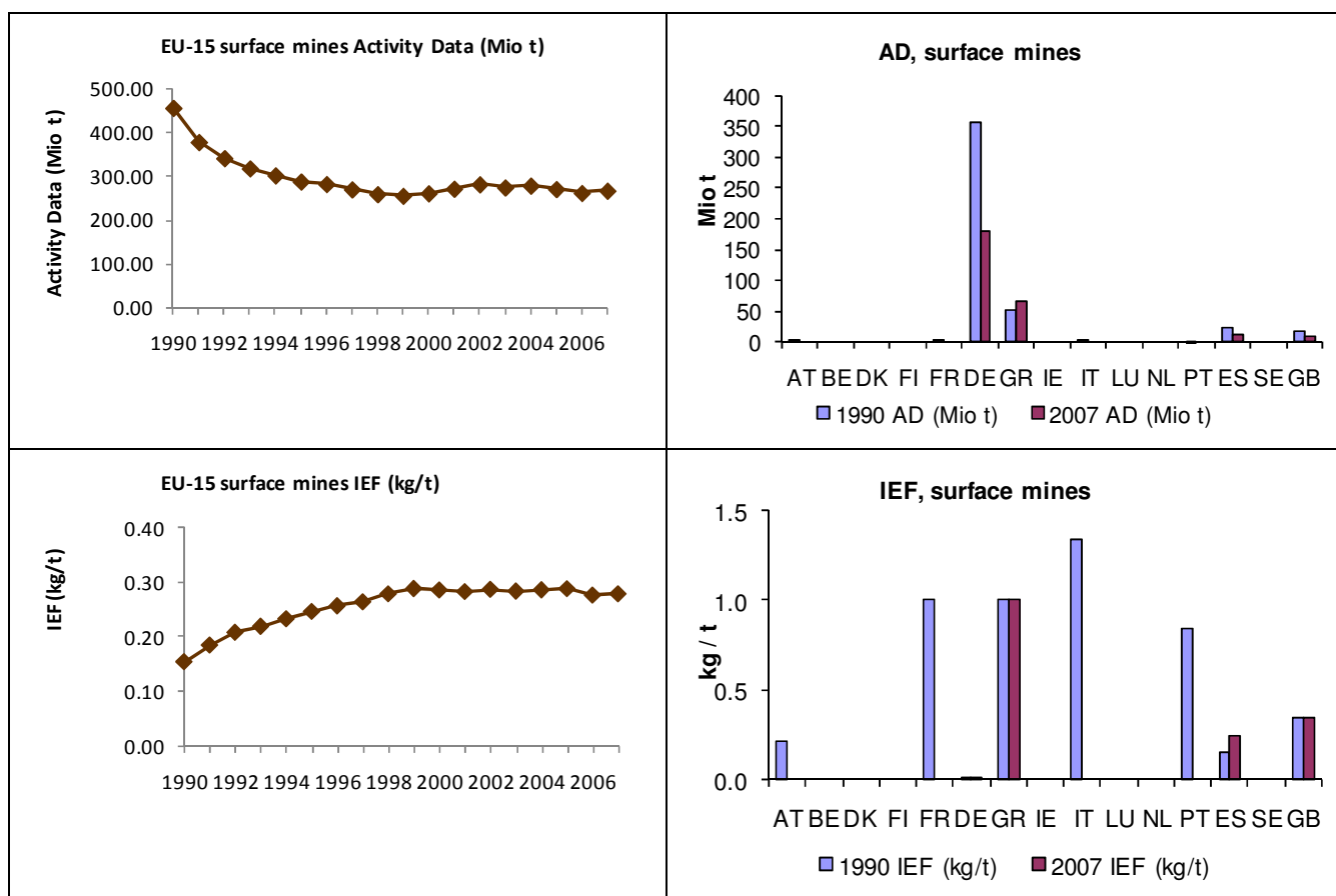
Figure 3.91 1B1aii Surface Mines: Activity Data and Implied Emission Factors for EU-15 and the emitting countries of CH 4
