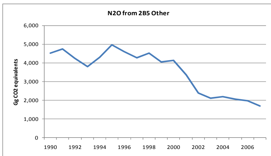
Figure 4.10 2B5 Other: EU-15 N 2 O emissions
