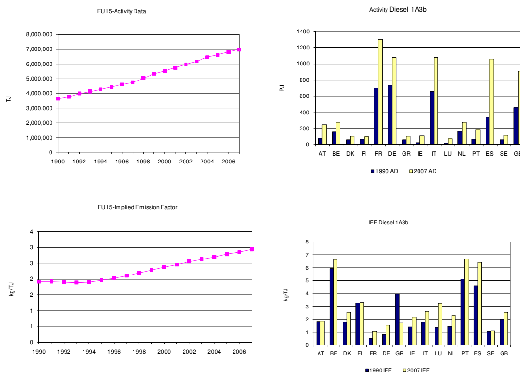
Figure 3.59 1A3b Road Transport, diesel oil: Activity Data and Implied Emission Factor for N 2 O emission
