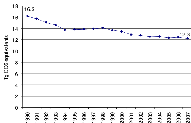
Figure 5.3 Sector 3 Solvent and Other Product Use: EU-27 GHG emissions for 1990–2007 in CO 2 equivalents (Tg)
